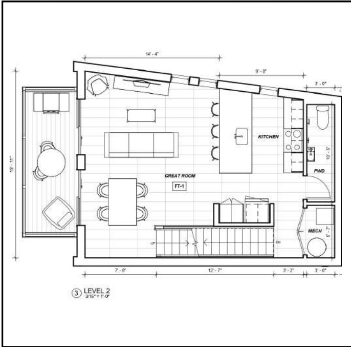
2nd Floor
